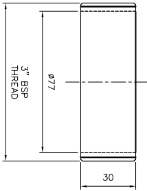
(SCALE:1:4) DETAIL-A BUSH FOR COUPLER
